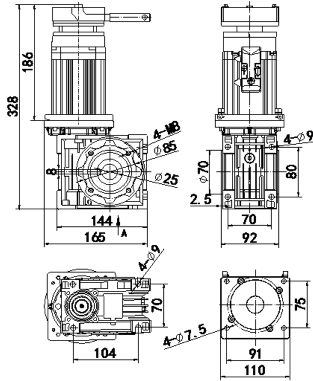
0.75KW Motor
