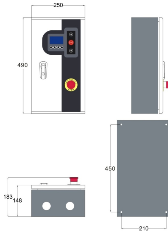
2.2KW Controller
